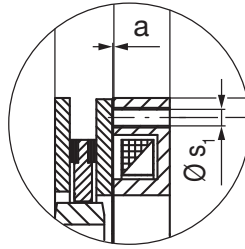
Type 8982.00001 Screw connection on the coil carrier back side
